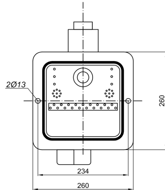
Assembly hole dimensions
